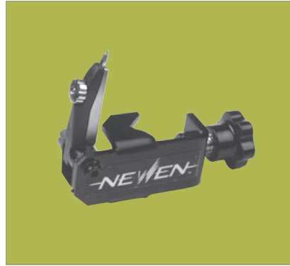
■ NWN-TSFA High precision tool setting fixture with interchangeable point.
